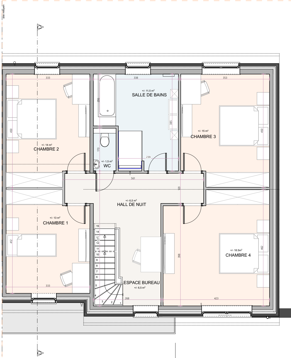
Etage lot 3
