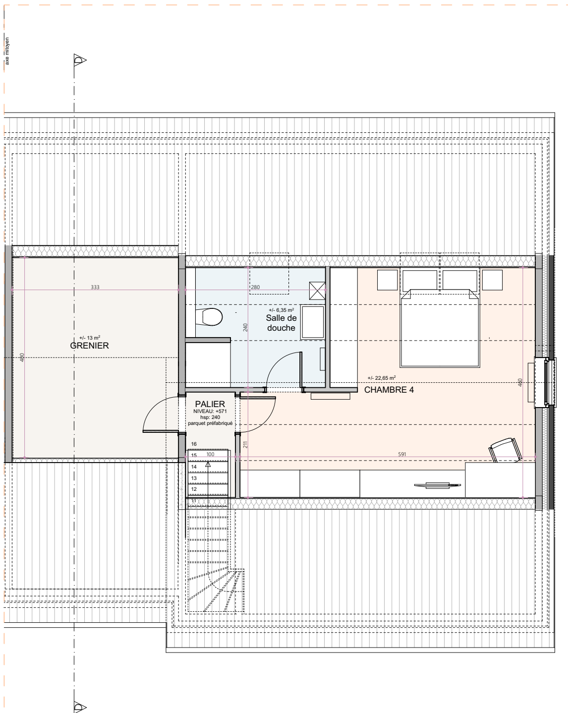
Combles lot 3
